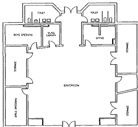
SCHOOL BUILDING LAYOUT JASPER MIDDLE SCHOOL BANDROOM BUILDING PICKENS COUNTY BOARD OF EDUCATION
