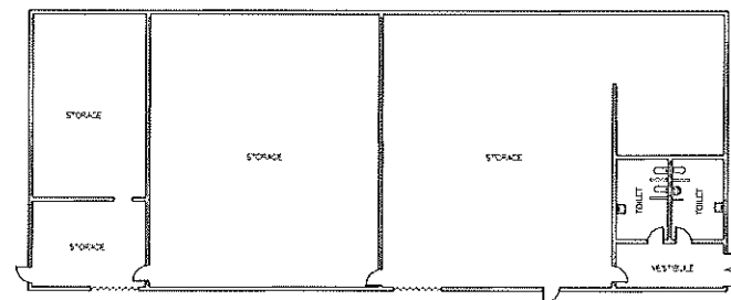
FIELD HOUSE BUILDING LAYOUT JASPER MIDDLE SCHOOL FIELD HOUSE LOWER LEVEL PICKENS COUNTY BOARD OF EDUCATION
